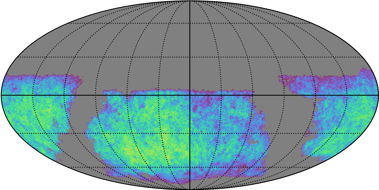
roll_uniform_early_half_mjdp180_v3.4_10yrs i band non-DD year 1: ExgalM5WithCuts
