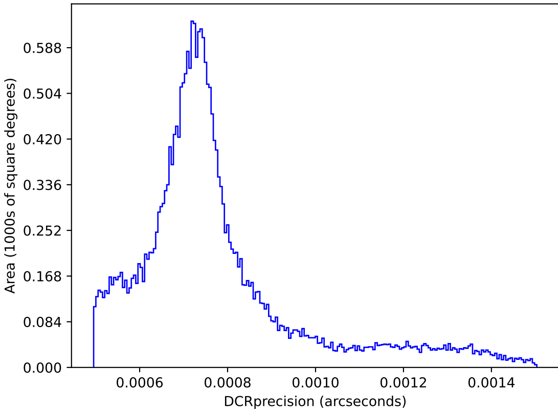
roll_uniform_early_half_mjdp180_v3.4_10yrs : DCRprecision
