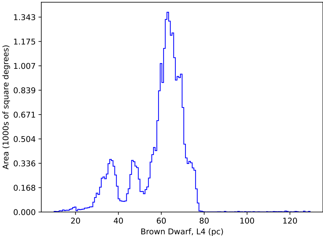
roll_uniform_early_half_mjdp180_v3.4_10yrs : Brown Dwarf, L4
