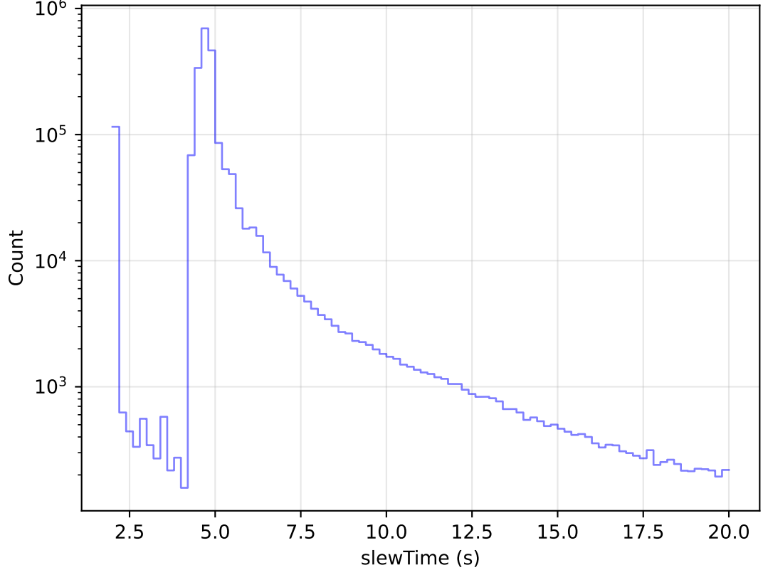
roll_uniform_early_half_mjdp180_v3.4_10yrs All visits: Zoom Slew Time Histogram
