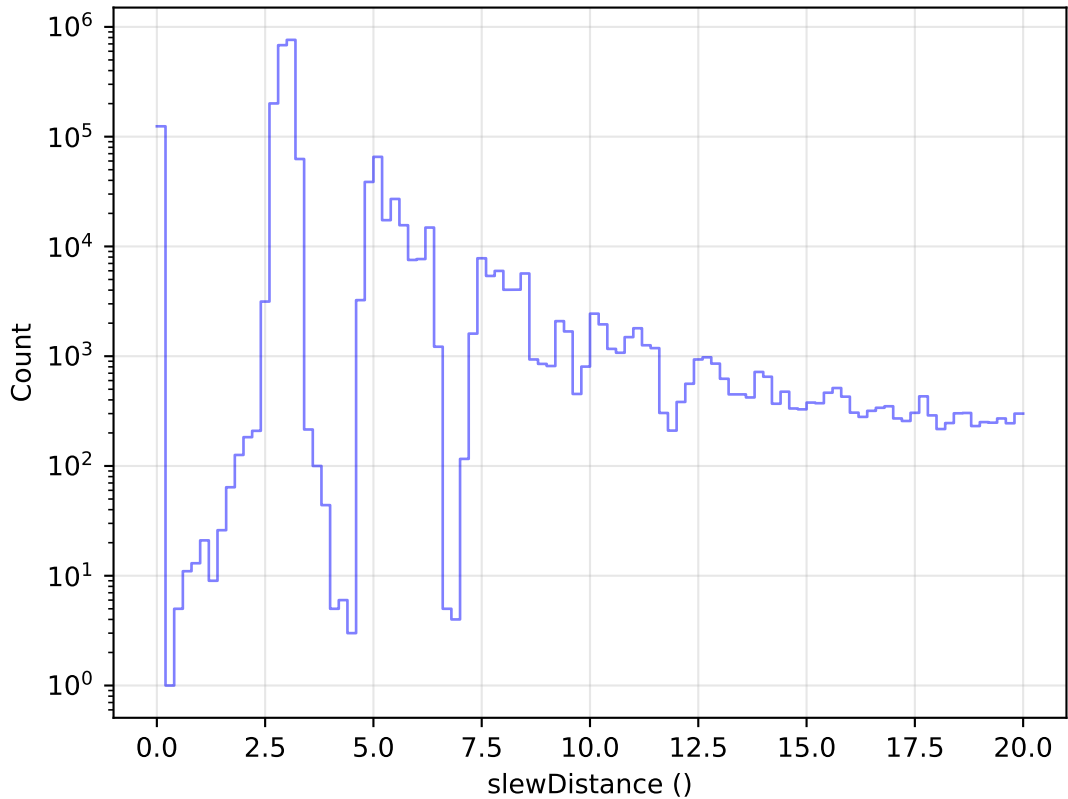
roll_uniform_early_half_mjdp180_v3.4_10yrs All visits: Zoom Slew Distance Histogram
