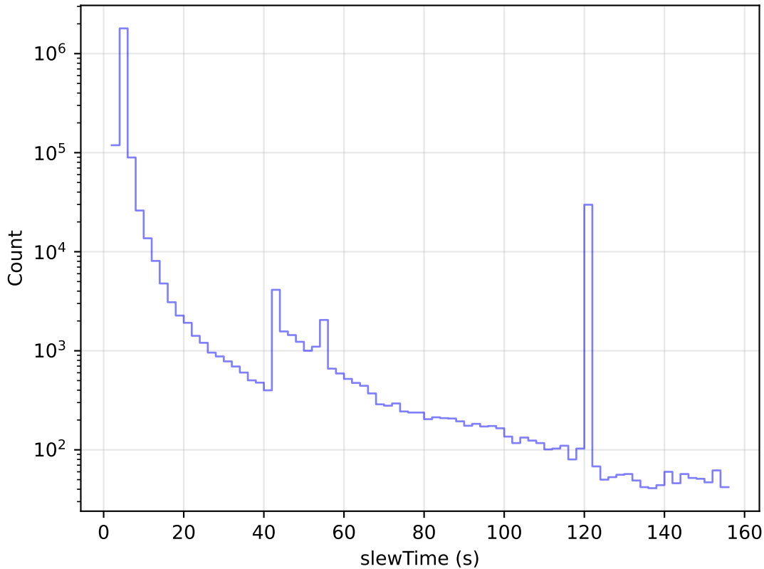
roll_uniform_early_half_mjdp180_v3.4_10yrs All visits: Slew Time Histogram
