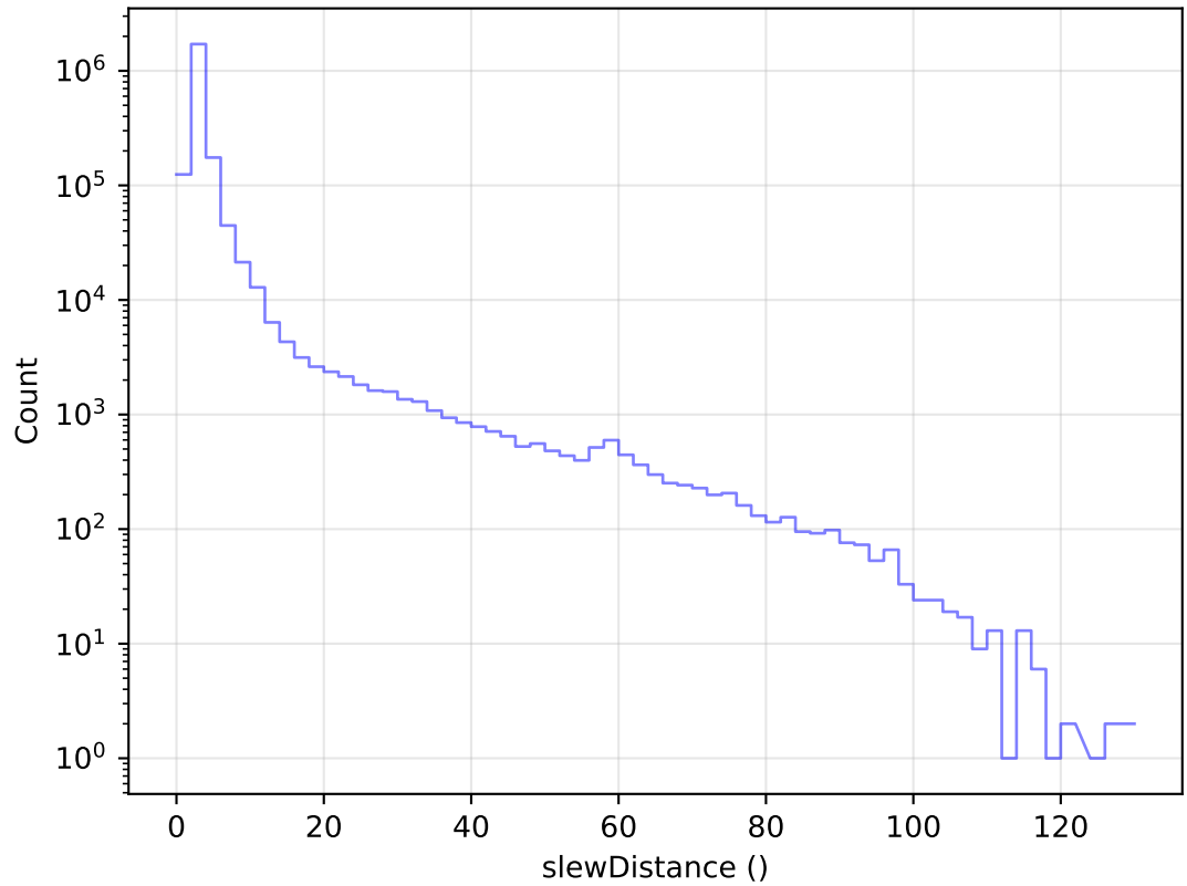
roll_uniform_early_half_mjdp180_v3.4_10yrs All visits: Slew Distance Histogram
