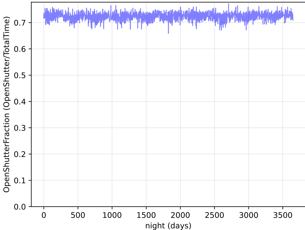
roll_uniform_early_half_mjdp180_v3.4_10yrs : OpenShutterFraction
