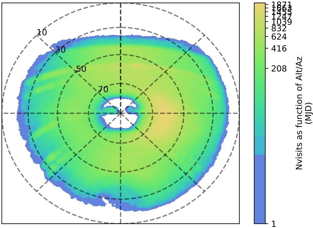
roll_uniform_early_half_mjdp180_v3.4_10yrs y: Nvisits as function of Alt/Az
