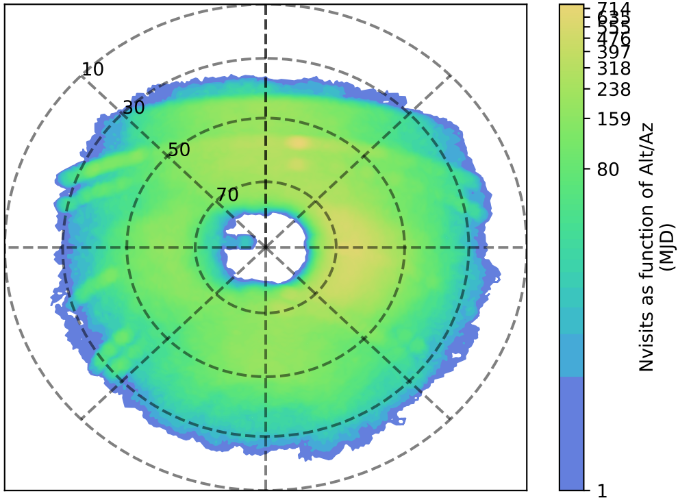
roll_uniform_early_half_mjdp180_v3.4_10yrs u: Nvisits as function of Alt/Az
