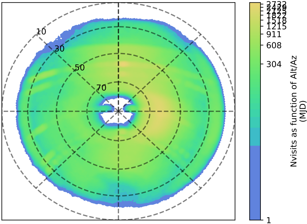
roll_uniform_early_half_mjdp180_v3.4_10yrs i: Nvisits as function of Alt/Az
