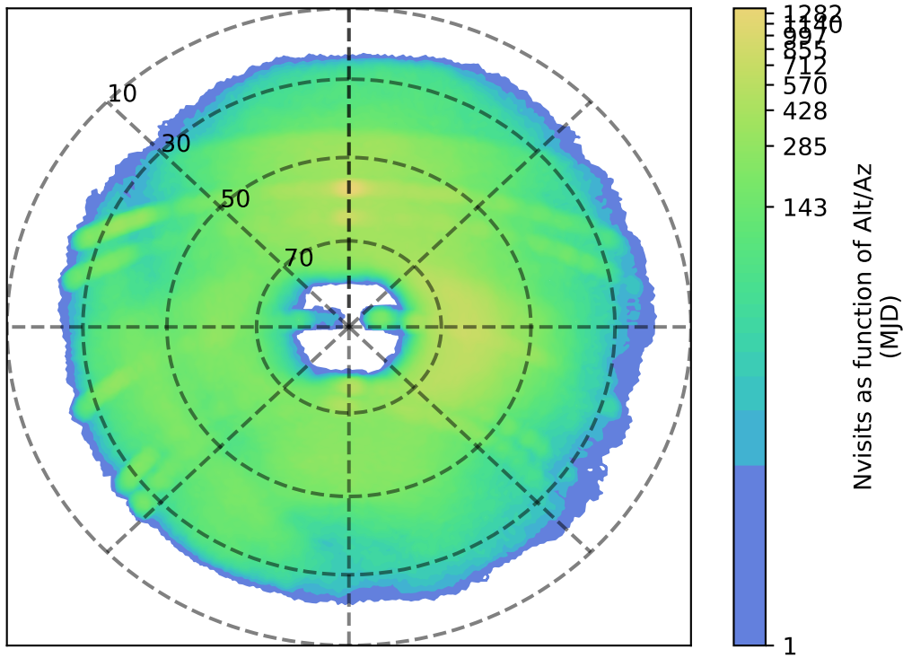
roll_uniform_early_half_mjdp180_v3.4_10yrs g: Nvisits as function of Alt/Az
