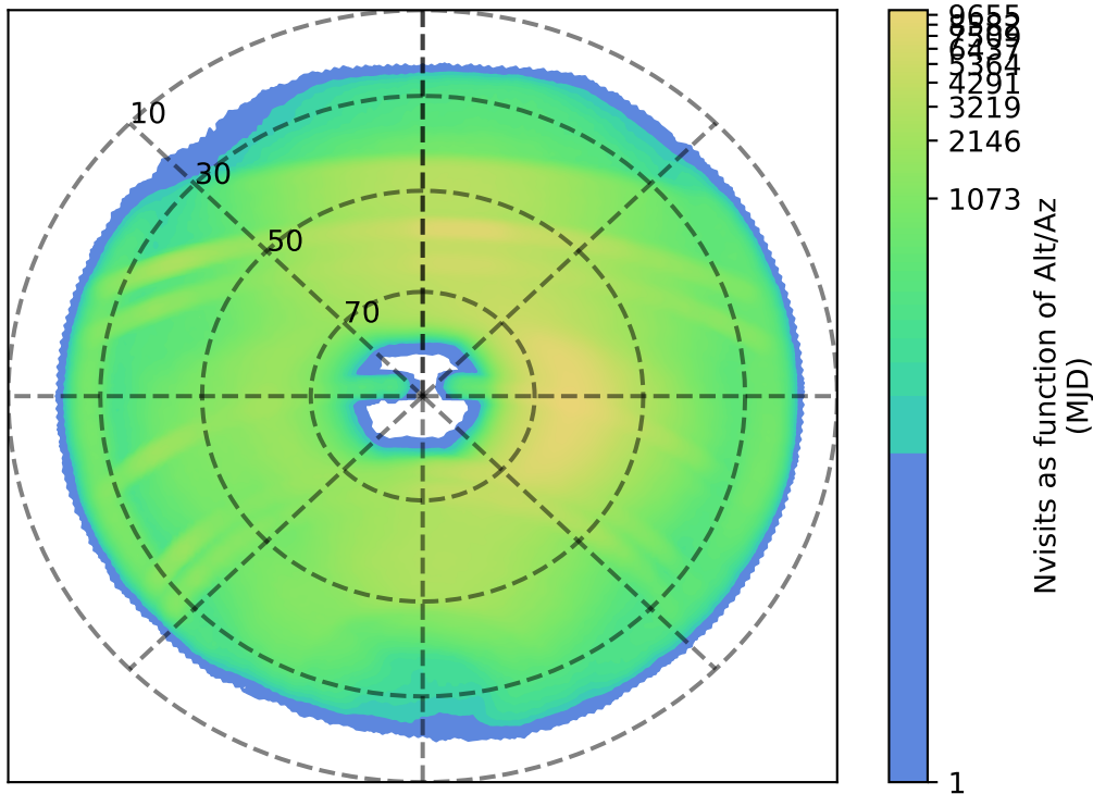
roll_uniform_early_half_mjdp180_v3.4_10yrs : Nvisits as function of Alt/Az
