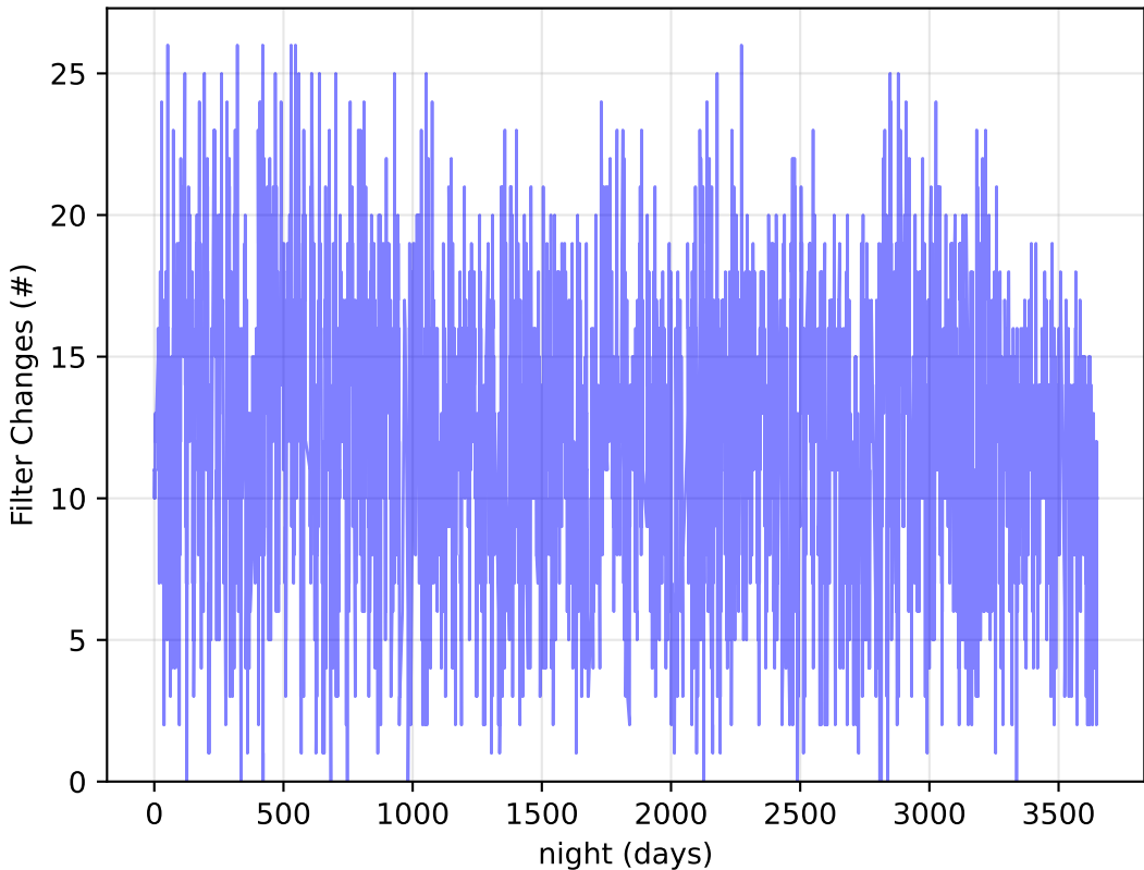
roll_uniform_early_half_mjdp180_v3.4_10yrs : Filter Changes
