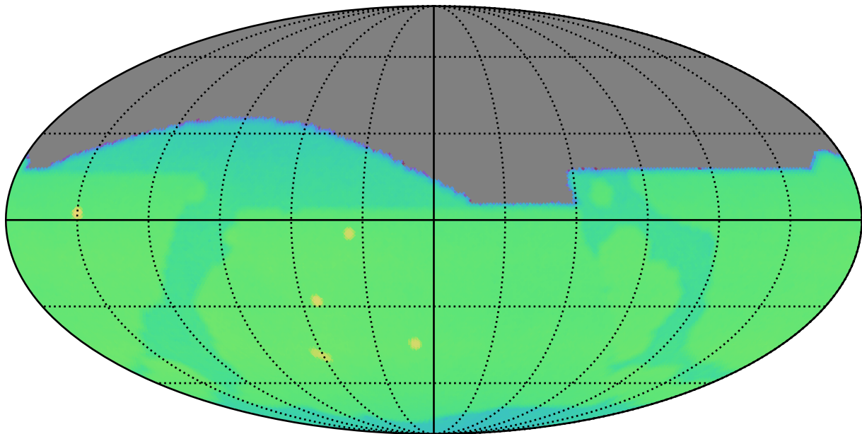
roll_uniform_early_half_mjdp180_v3.4_10yrs : CoaddM5
