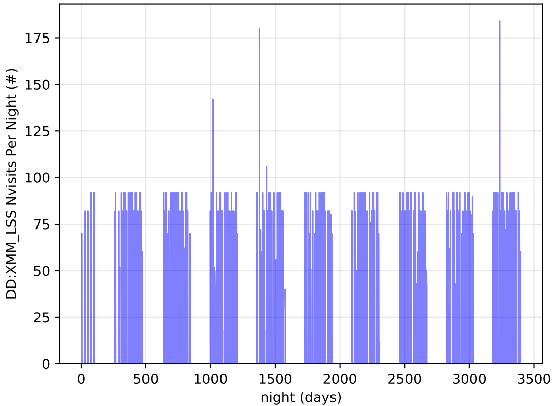
roll_uniform_early_half_mjdp180_v3.4_10yrs all bands: DD:XMM_LSS Nvisits Per Night
