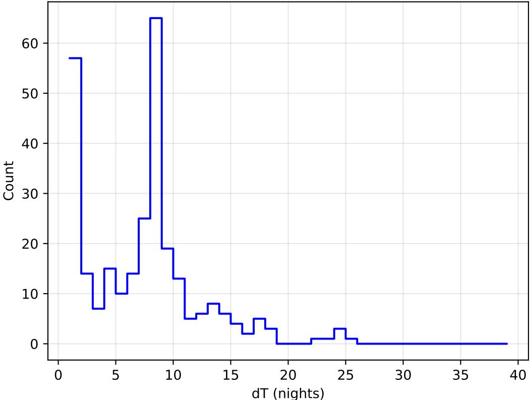
roll_uniform_early_half_mjdp180_v3.4_10yrs all bands: DD:XMM_LSS Delta Nights Histogram
