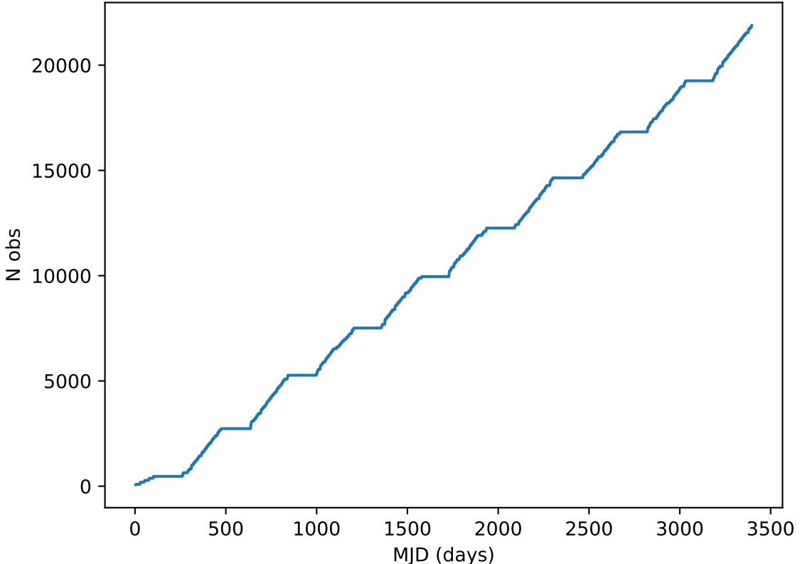
roll_uniform_early_half_mjdp180_v3.4_10yrs all bands: DD:XMM_LSS Cumulative NVisits
