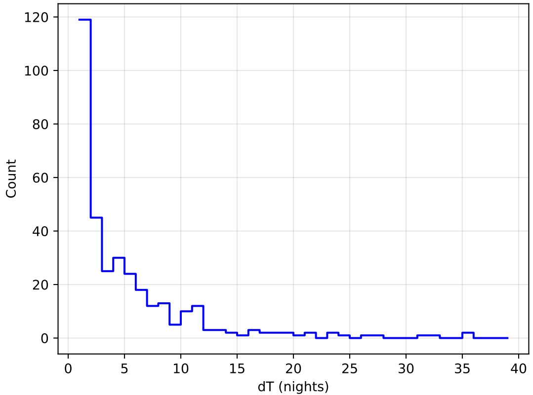
roll_uniform_early_half_mjdp180_v3.4_10yrs all bands: DD:WFD Delta Nights Histogram
