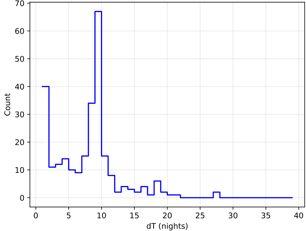
roll_uniform_early_half_mjdp180_v3.4_10yrs all bands: DD:ELAISS1 Delta Nights Histogram
