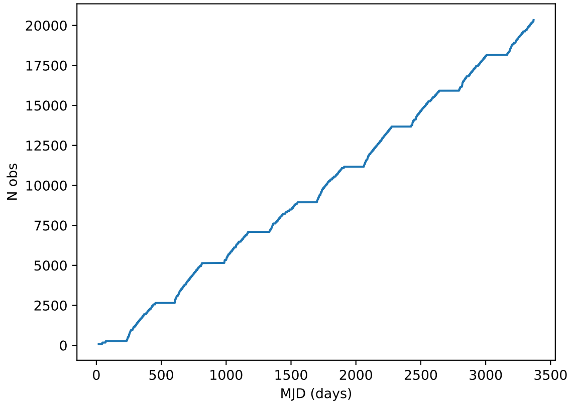
roll_uniform_early_half_mjdp180_v3.4_10yrs all bands: DD:ELAISS1 Cumulative NVisits
