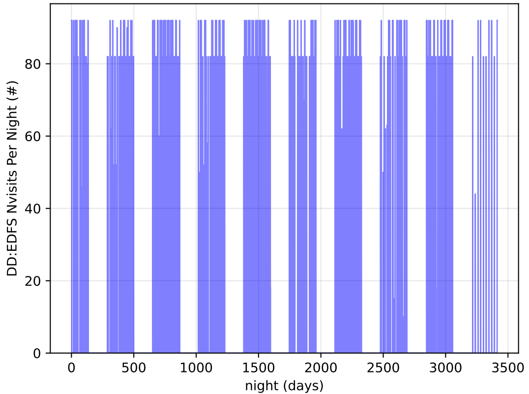
roll_uniform_early_half_mjdp180_v3.4_10yrs all bands: DD:EDFS Nvisits Per Night
