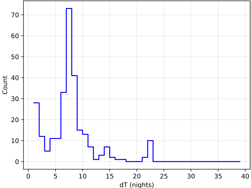
roll_uniform_early_half_mjdp180_v3.4_10yrs all bands: DD:EDFS Delta Nights Histogram
