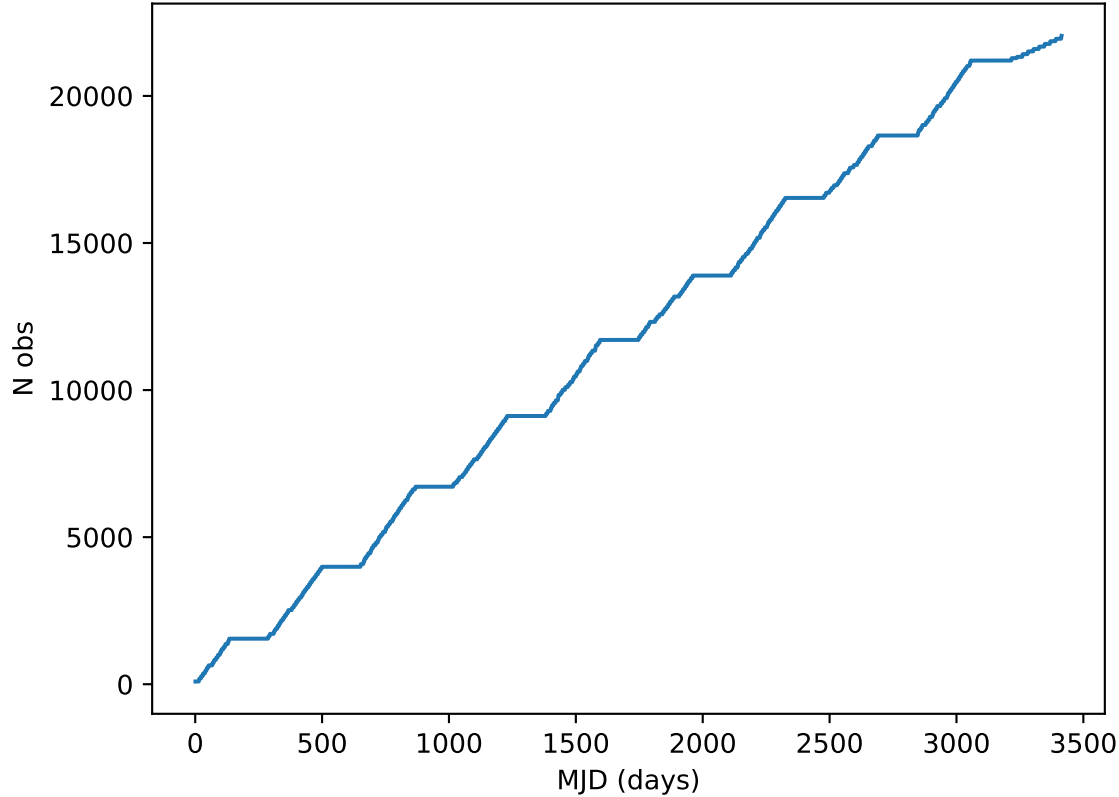
roll_uniform_early_half_mjdp180_v3.4_10yrs all bands: DD:EDFS Cumulative NVisits
