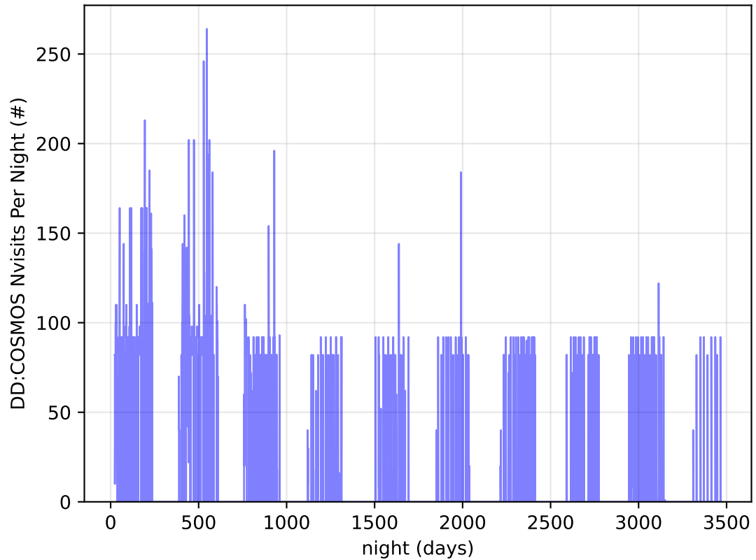
roll_uniform_early_half_mjdp180_v3.4_10yrs all bands: DD:COSMOS Nvisits Per Night
