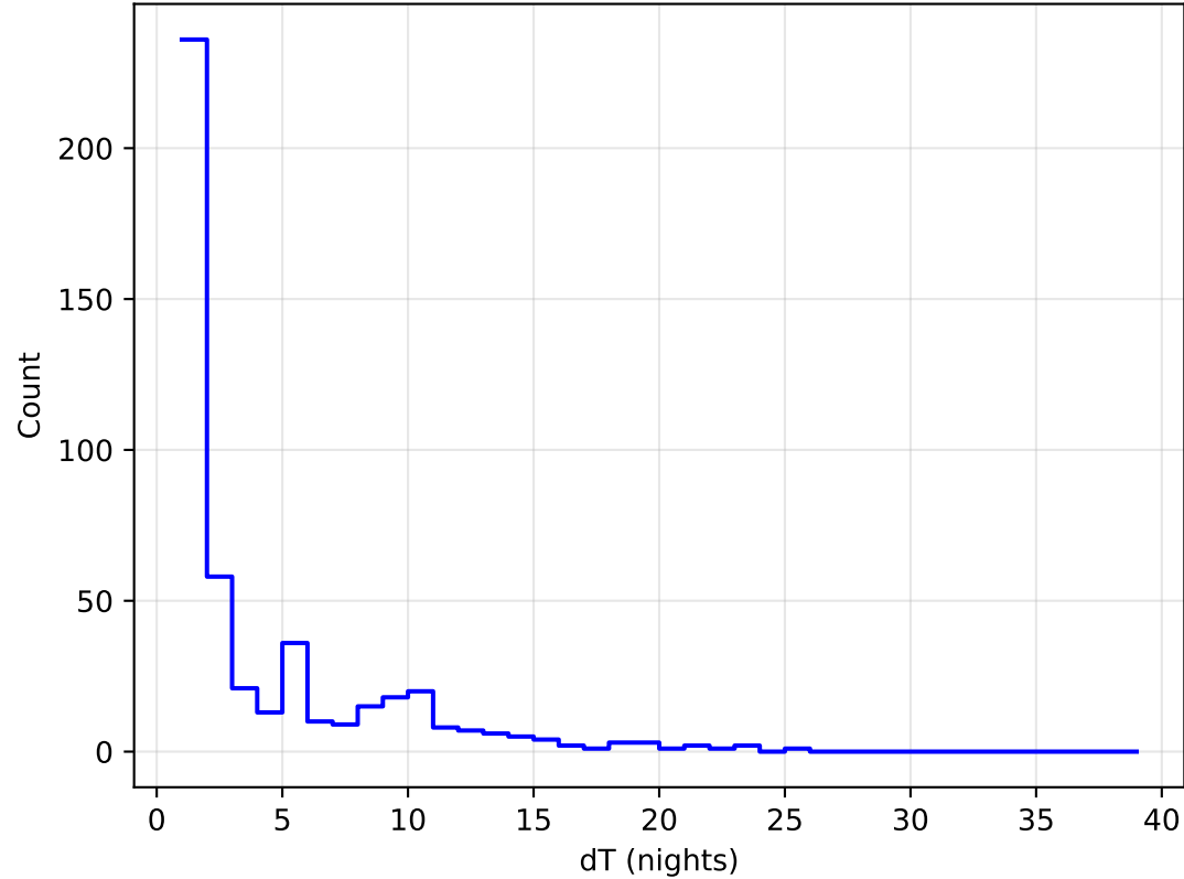
roll_uniform_early_half_mjdp180_v3.4_10yrs all bands: DD: COSMOS Delta Nights Histogram
