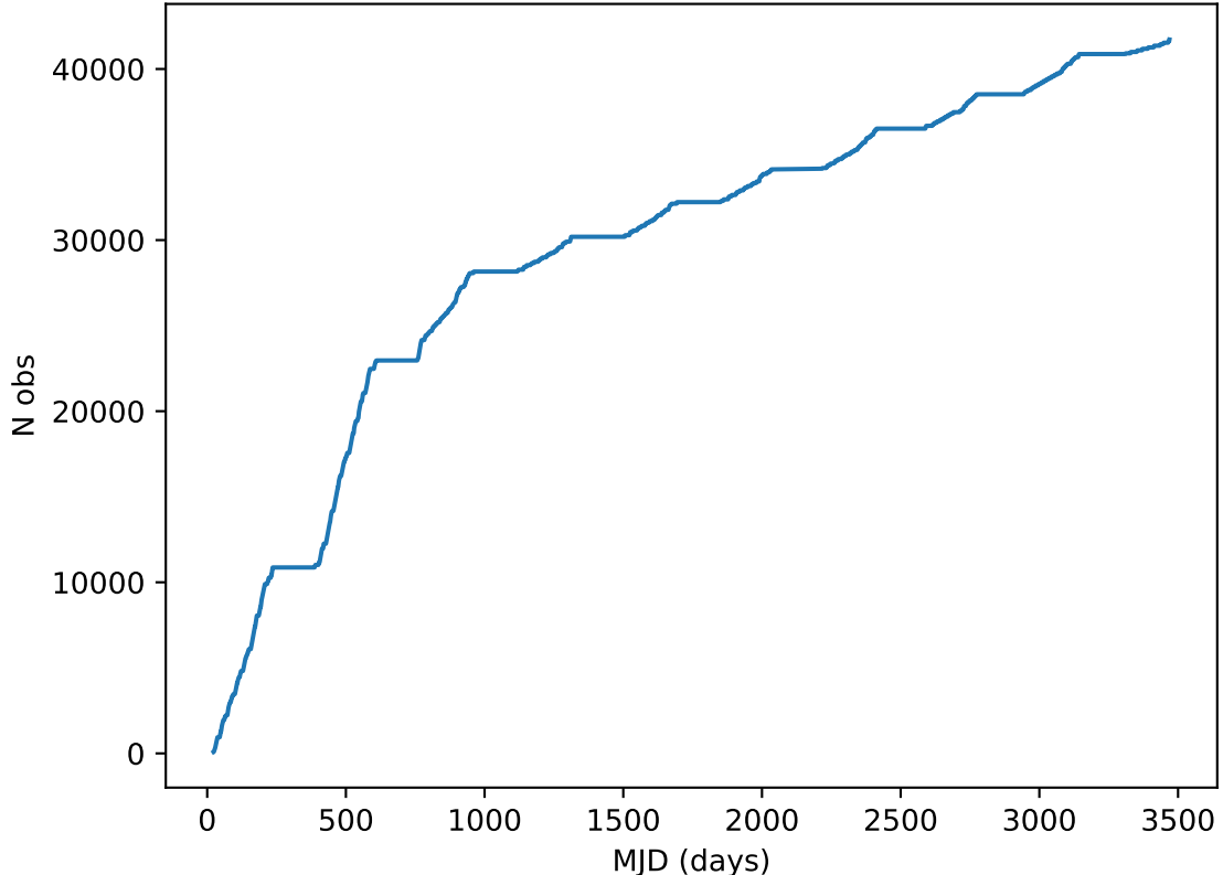
roll_uniform_early_half_mjdp180_v3.4_10yrs all bands: DD: COSMOS Cumulative NVisits
