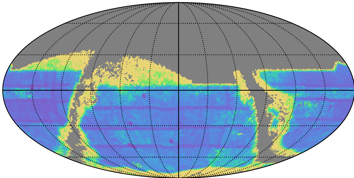
roll_uniform_early_half_mjdp0_v3.4_10yrs : TDC_precision
