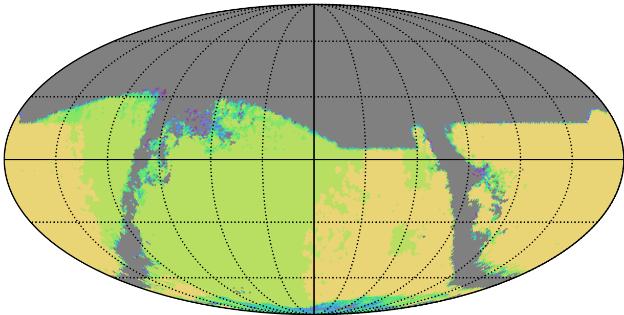
roll_uniform_early_half_mjdp0_v3.4_10yrs : TDC_campaign
