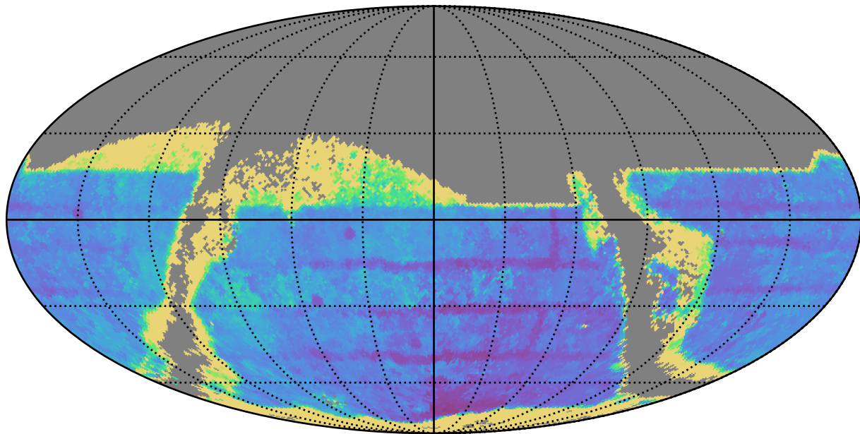
roll_uniform_early_half_mjdp0_v3.4_10yrs : TDC_accuracy
