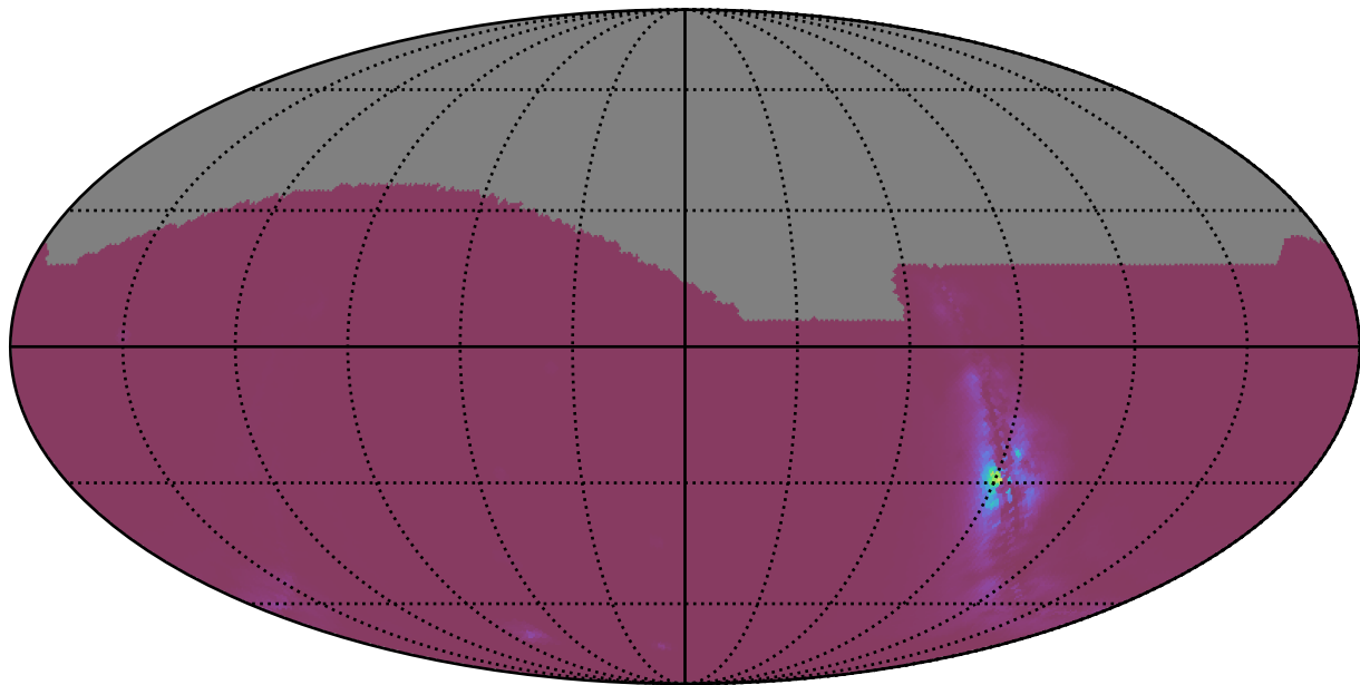
roll_uniform_early_half_mjdp0_v3.4_10yrs : NlcPoints
