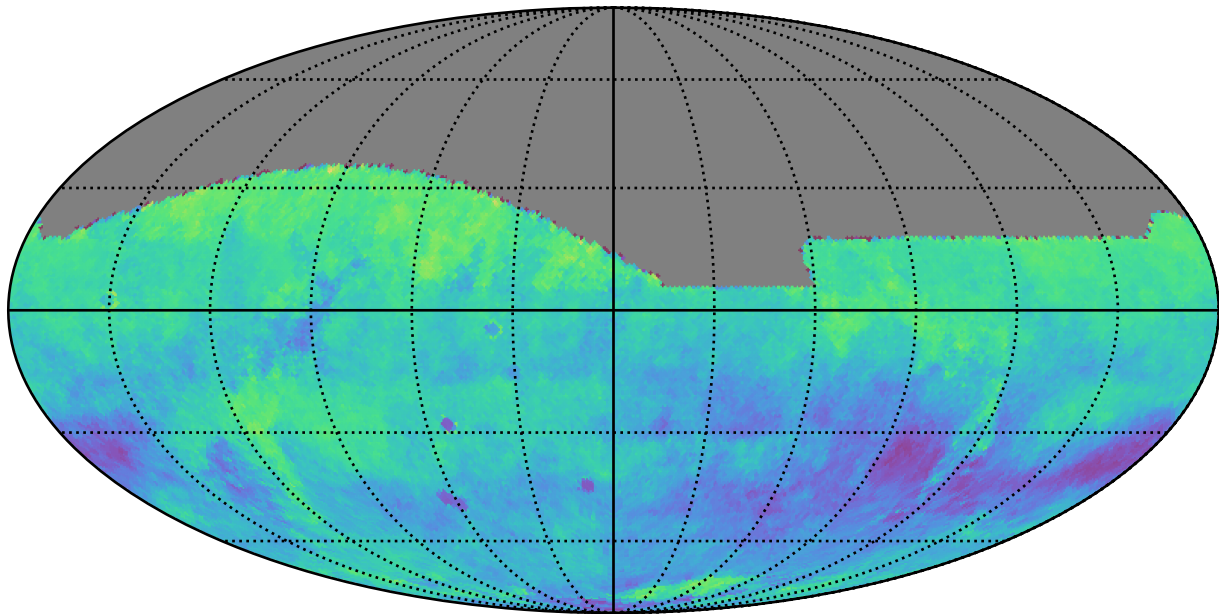
roll_uniform_early_half_mjdp0_v3.4_10yrs z: Kuiper rotSkyPos
