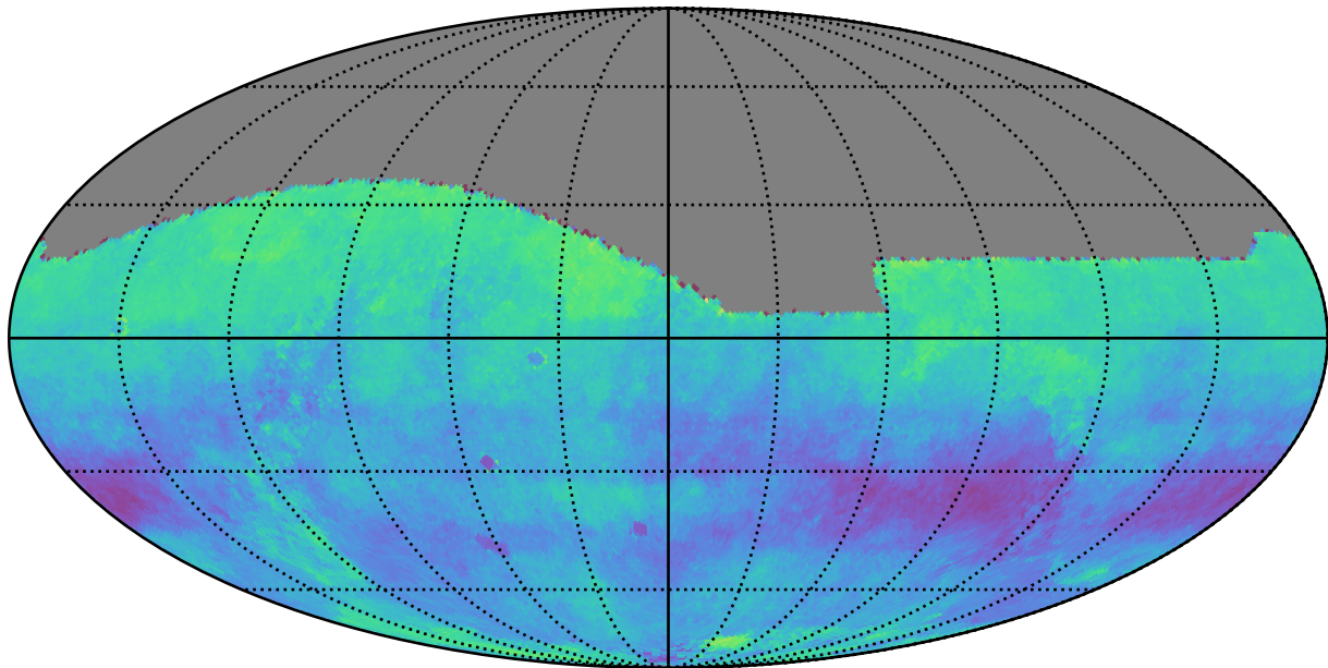
roll_uniform_early_half_mjdp0_v3.4_10yrs r: Kuiper rotSkyPos
