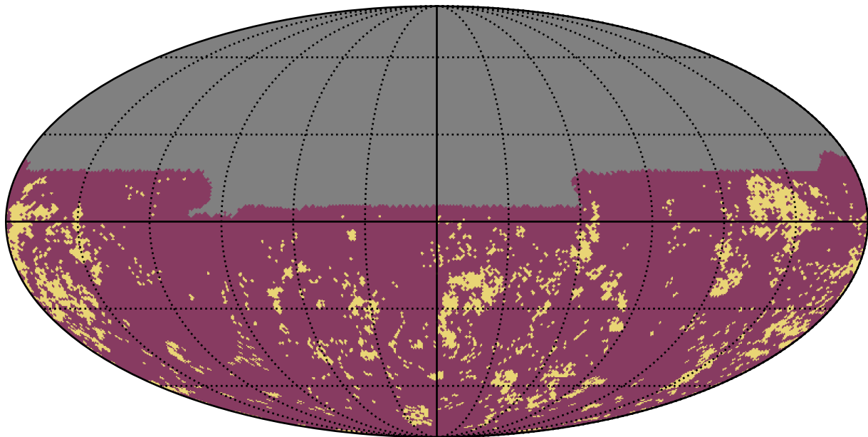
roll_uniform_early_half_mjdp0_v3.4_10yrs u band: Gaps_3hr
