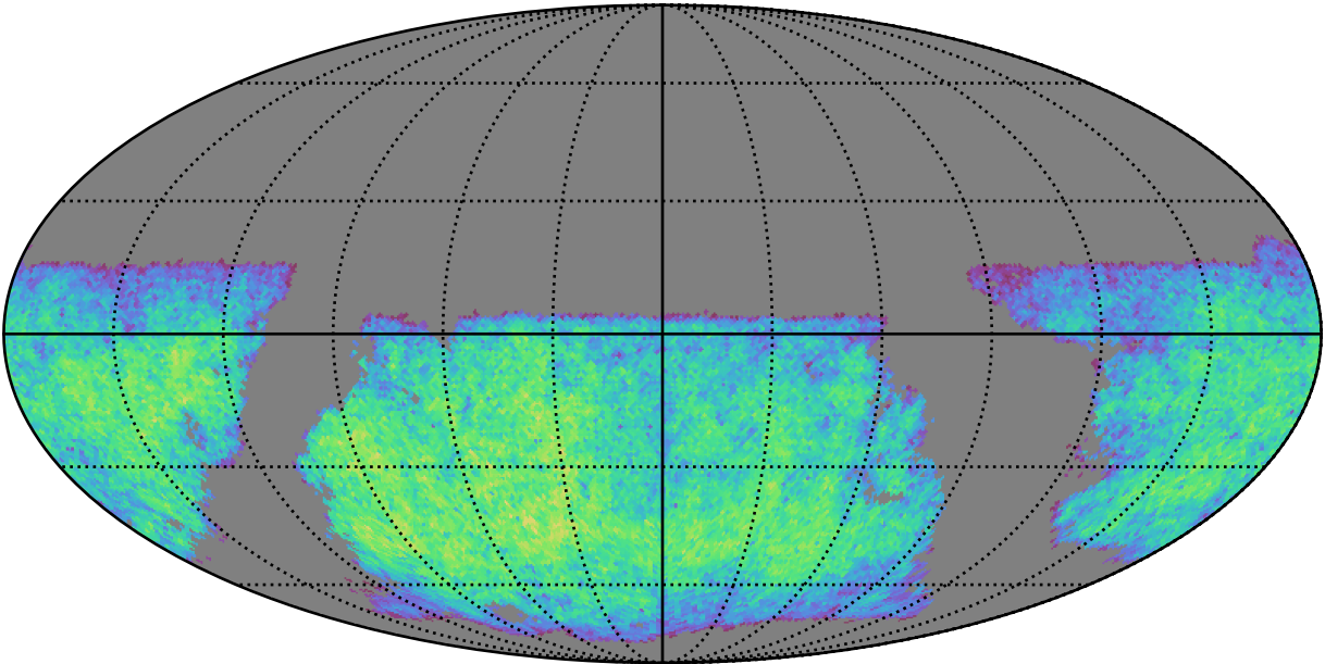
roll_uniform_early_half_mjdp0_v3.4_10yrs i band non-DD year 1: ExgalM5WithCuts
