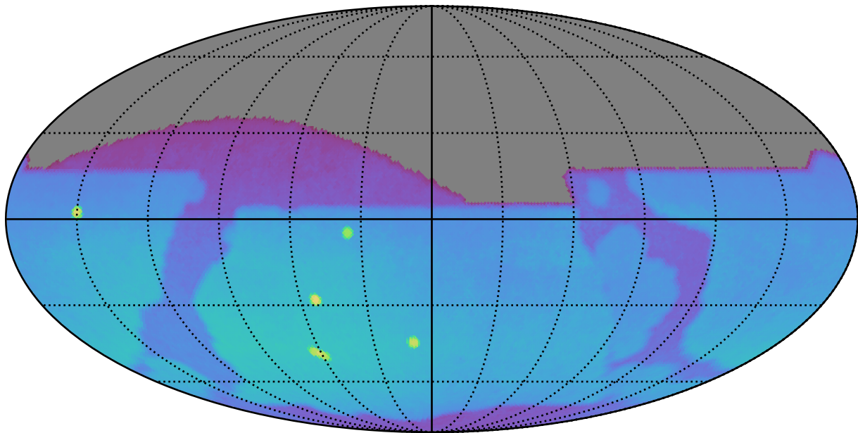
roll_uniform_early_half_mjdp0_v3.4_10yrs : Brown Dwarf, L7
