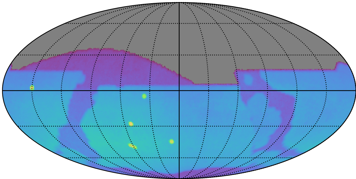
roll_uniform_early_half_mjdp0_v3.4_10yrs : Brown Dwarf, L4
