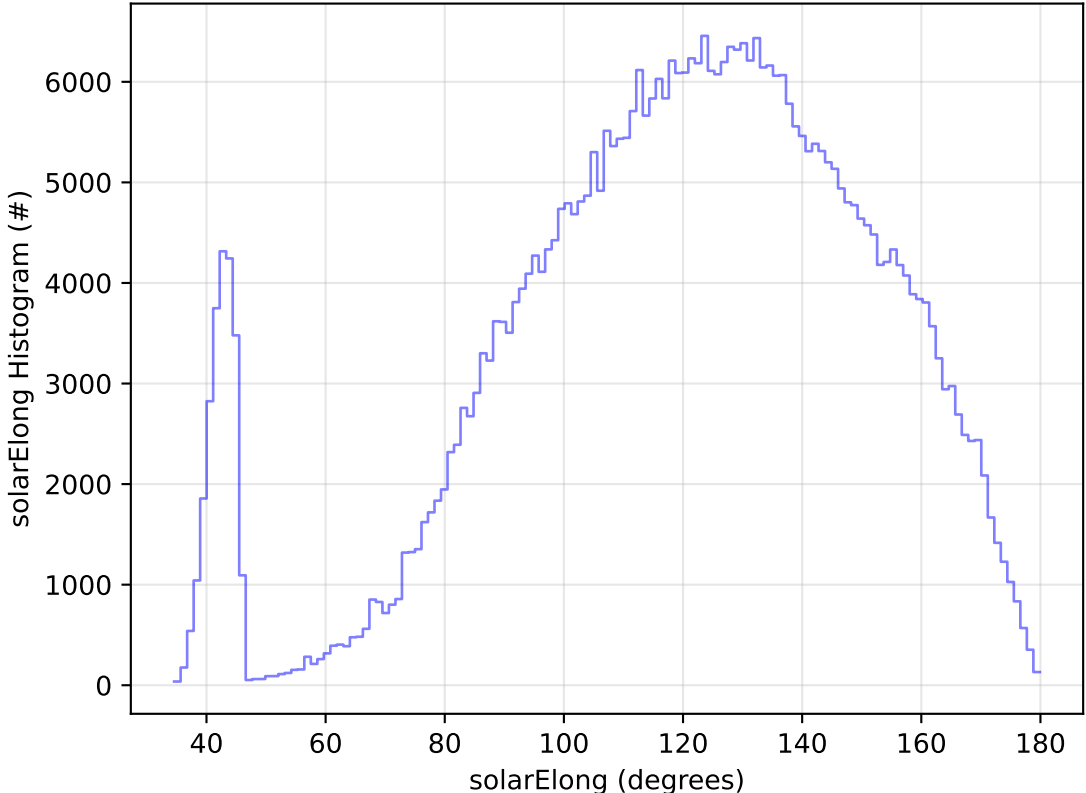
roll_uniform_early_half_mjdp0_v3.4_10yrs WFD z band: solarElong Histogram
