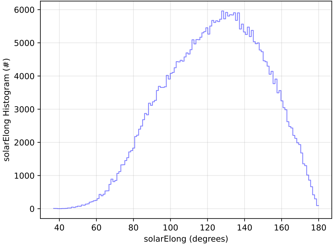
roll_uniform_early_half_mjdp0_v3.4_10yrs WFD y band: solarElong Histogram
