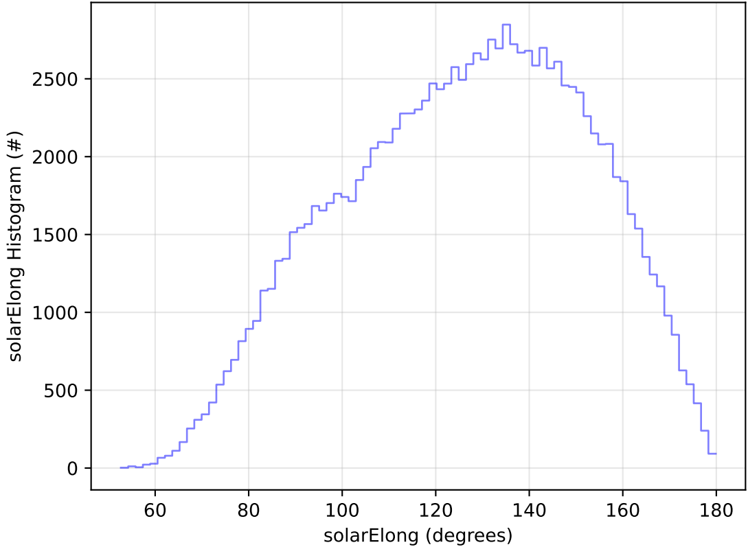
roll_uniform_early_half_mjdp0_v3.4_10yrs WFD u band: solarElong Histogram
