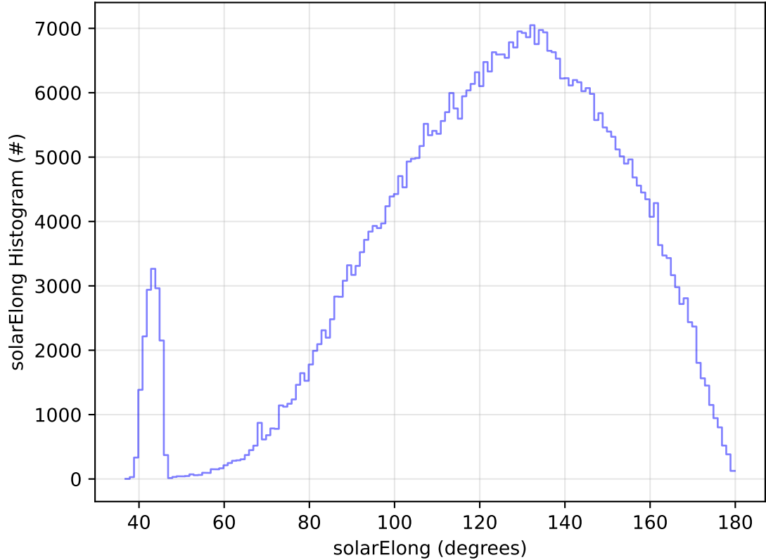
roll_uniform_early_half_mjdp0_v3.4_10yrs WFD r band: solarElong Histogram
