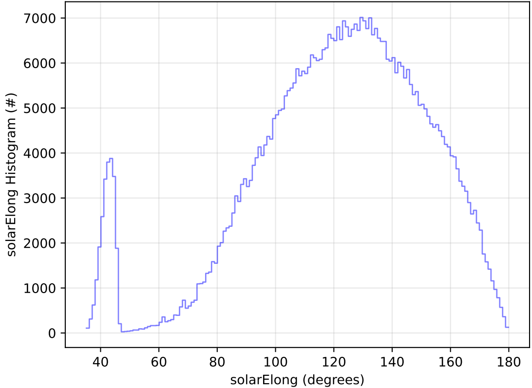
roll_uniform_early_half_mjdp0_v3.4_10yrs WFD i band: solarElong Histogram
