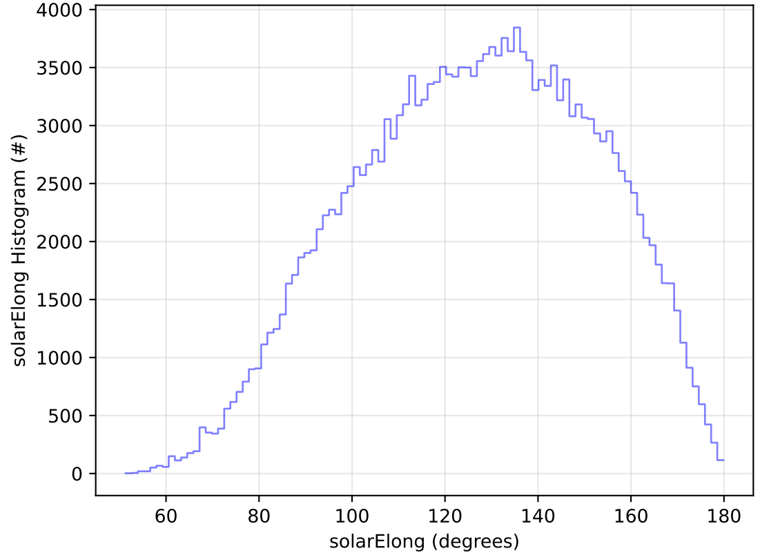
roll_uniform_early_half_mjdp0_v3.4_10yrs WFD g band: solarElong Histogram
