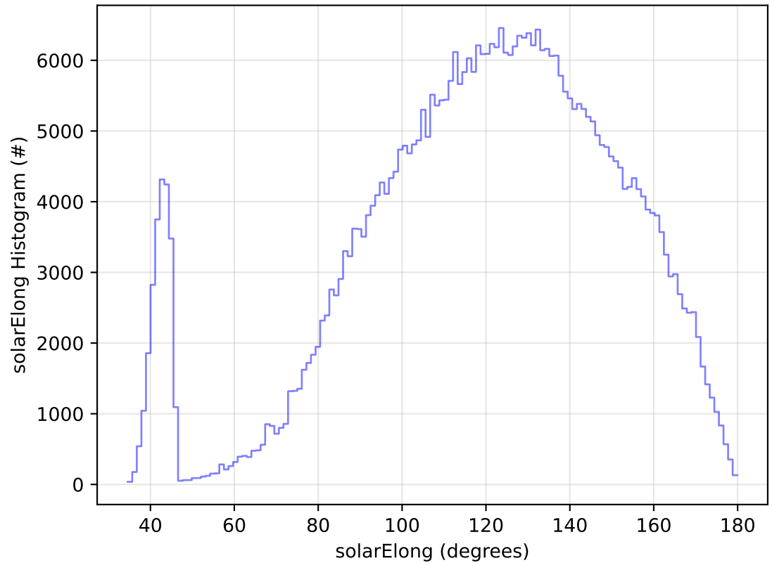
roll_uniform_early_half_mjdp0_v3.4_10yrs All sky z band: solarElong Histogram
