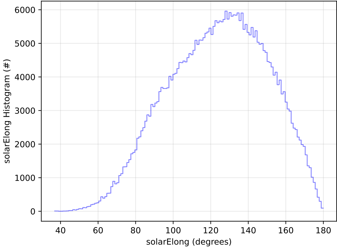
roll_uniform_early_half_mjdp0_v3.4_10yrs All sky y band: solarElong Histogram
