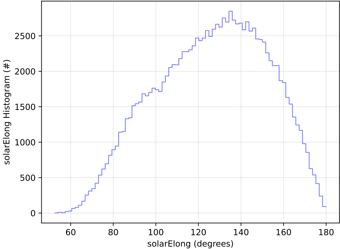
roll_uniform_early_half_mjdp0_v3.4_10yrs All sky u band: solarElong Histogram
