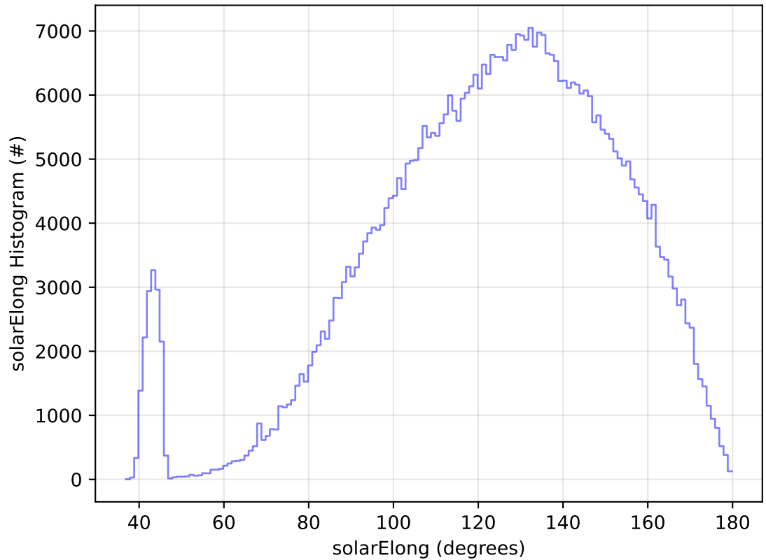
roll_uniform_early_half_mjdp0_v3.4_10yrs All sky r band: solarElong Histogram
