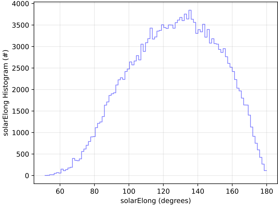
roll_uniform_early_half_mjdp0_v3.4_10yrs All sky g band: solarElong Histogram
