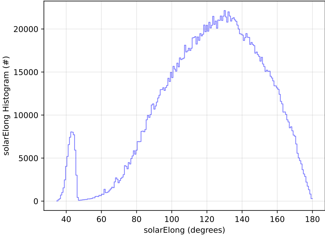
roll_uniform_early_half_mjdp0_v3.4_10yrs All sky all bands: solarElong Histogram
