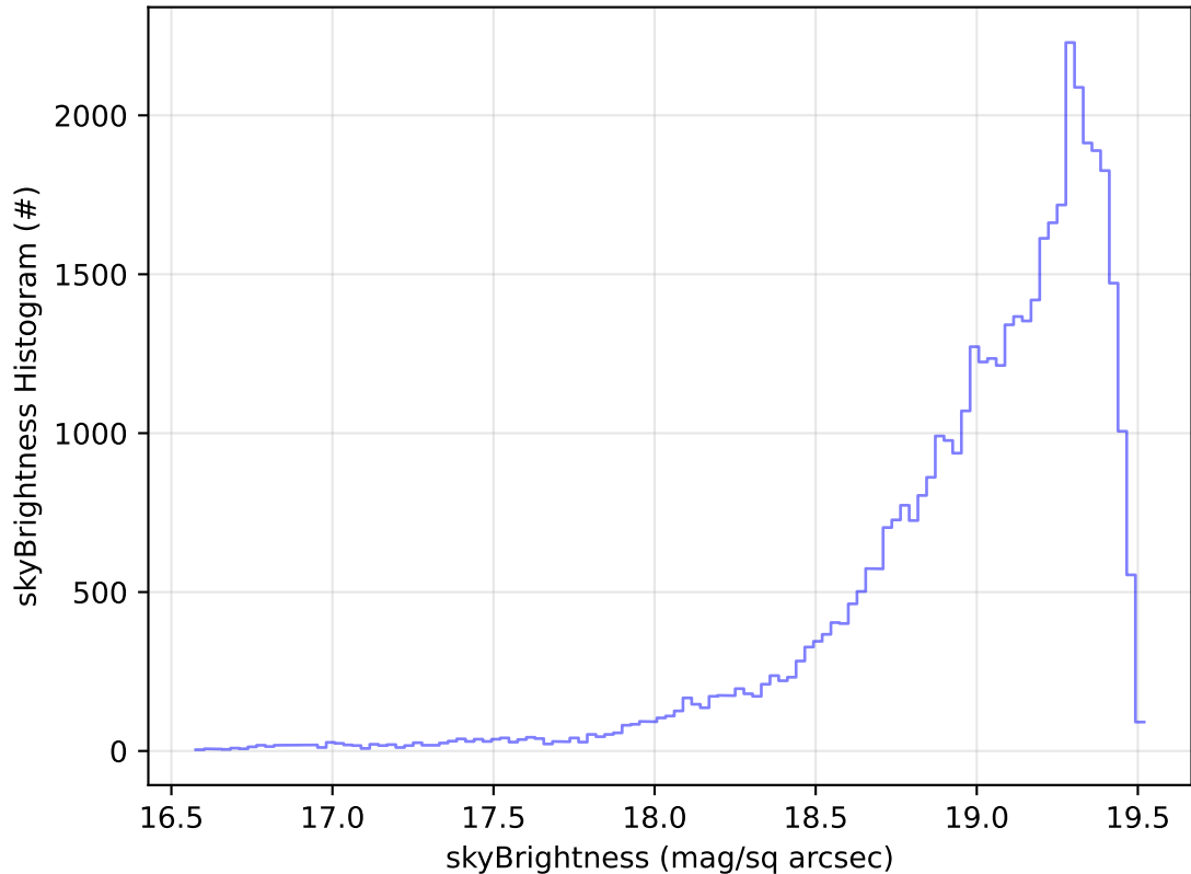
roll_uniform_early_half_mjdp0_v3.4_10yrs Yr 1 z band: skyBrightness Histogram
